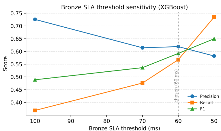
Figure 5.2: Precision, recall, and F1 across candidate Bronze SLA thresholds.
